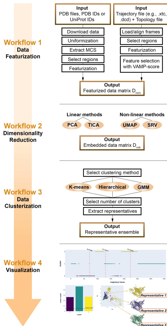
Figure 1: Overview of the EnGens methodology. Workflows are listed across the vertical arrow on the left. Individual steps are listed in the diagram on the right.
