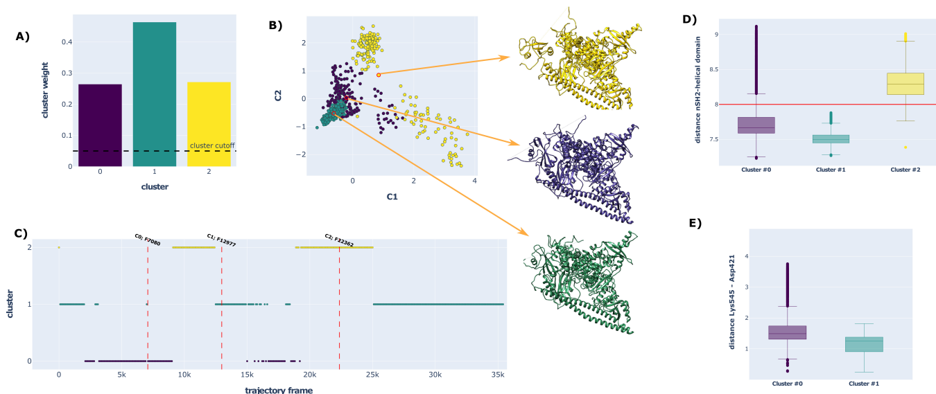
Figure 3: EnGen processing of the Galdadas et al. MD trajectory of PI3K. A) The proportion belonging to each cluster is plotted on the y-axis (cluster weight). Cluster indexes are listed on the x-axis. B) Two-dimensional embedding based on the components identified by the SRV method. Datapoints represent frames and are colored based on their respective cluster (same colors as in A). The 3D structural models of the three cluster representatives are shown on the right of this plot. C) The timeline view of the trajectory, where the x-axis lists the index of each frame, and the y-axis lists the corresponding cluster index. Vertical red lines highlight the representative frames extracted in the generated ensemble. D) The distance between nSH2 and the helical domain of PI3K is plotted on the y-axis. The x-axis lists the clusters. The red horizontal line represents the threshold of 8 Å. E) The distance between Lys545 and Asp421 of the PI3K regulatory unit is plotted on the y-axis. The x-axis lists the clusters.
