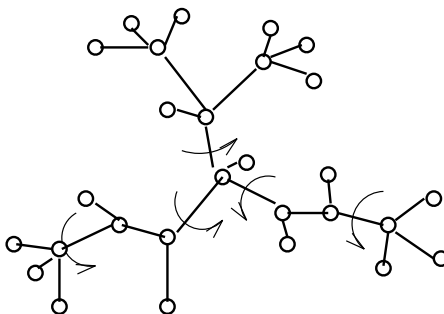
Fig. 2. The molecule of valine with its torsional degrees of freedom. A ball indicates an atom center, and a line segment indicates a bond between two atoms.
