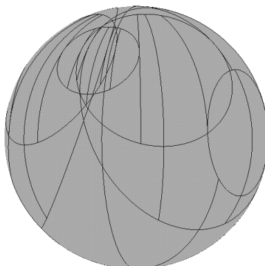
Fig. 1. Partial trapezoidal decomposition of an arrangement of small circles on an atom sphere.
