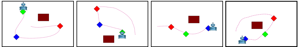
Fig. 3. A motivating example of the interface used in the human study. (Left:) Instructions specifying maroon obstacles, and ordering constraints for red( R ), blue( B ), and green( G ) diamonds. (Right four:) Our approach over 4 experiment examples with the snapshot showing the path (dotted pink) and the position of the robot at the end of the demonstration. The first is a random environment. The right three generate environments that a) are confident about maroon being global constraints, and b) place an informative permutation of goals ( GBR , RGB , BGR respectively) along an optimal path. Consider the second experiment. The current estimate supports B after R from the previous demonstration. The second environment is optimized to incentivize a demonstration with GBR . The fact that the demonstrator still chooses R before B is informative. Experiment design effectively makes inference converge.
