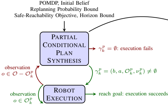
Fig. 3: The overall structure of the OPCPS Algorithm
